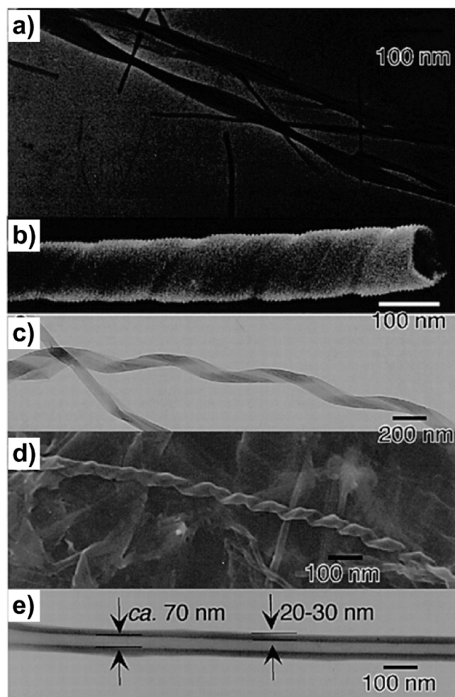
FIGURE 5. EF-TEM and SEM pictures of the self-assembled (a) PheGlu2, (b, c) PheGlu3, and (d, e) PheGlu4. Reprinted with permission from ref 37. Copyright 2002 American Chemical Society.
